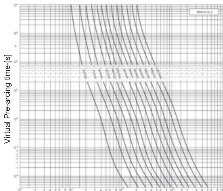
Time-Current Characteristics
