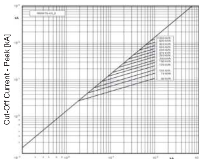
Cutoff Current Characteristics
